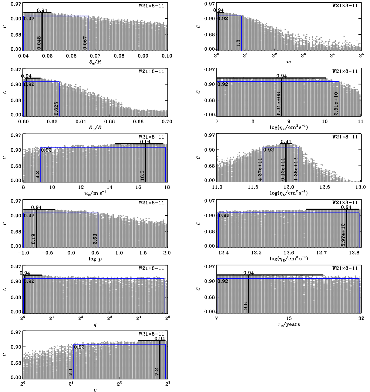
Figure 4. Same as Figure 2, but for the eleven model parameters ( \delta_c , R_b , u_0 , p , q , v , w , \eta_c , \eta_t , \eta_R , and \tau_R ), from four independent W21×8-11 optimisations, while the seven “emergence” parameters are held fixed to their optimal value listed in Table 1.
