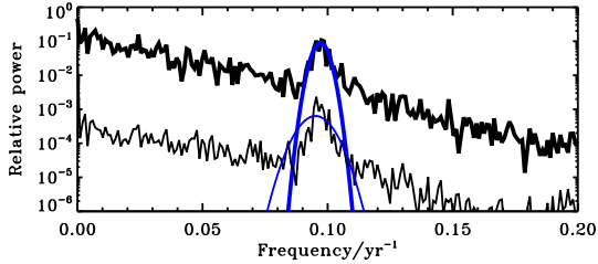
Figure 9. Relative spectra of the total magnetic energy (thick black) and pseudo-SSN (thin black) time series, averaged over three independent realizations of a \simeq 96 -cycles tilt-quenched 2 \times 2D dynamo simulation. Continuous blue curves illustrate the gaussian best fit to each spectrum.
