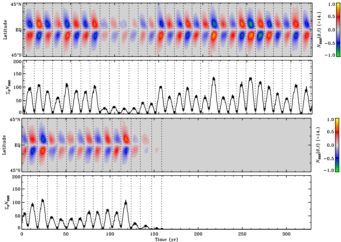
Figure 10. Time–latitude density plot (butterfly diagram) and corresponding monthly number (pseudo-SSN) of newly emerged BMRs, for two distinct realizations of a \simeq 32 -cycles tilt-quenched 2 \times 2D dynamo simulation using the same optimal parameter values used to produce the reference solution of Figure 7 (viz. panels (d) and (e)).
