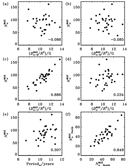
Figure 8. Amplitude (maximum pseudo-SSN) of cycle n as a function of maximum axial dipole moment at the end of (a) cycle n - 3 , (b) cycle n - 2 , (c) cycle n - 1 , and (d) cycle n , for the sample dynamo solution presented in Figure 7. (e) Cycle amplitude as compared to the period of the same cycle. (f) Cycle amplitude calculated independently in each hemisphere and plotted against one another. In each panel is also given the corresponding Pearson’s linear coefficient.
